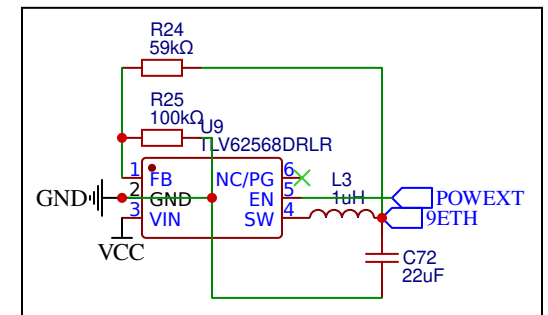
PWR Delivery - 0.9V
